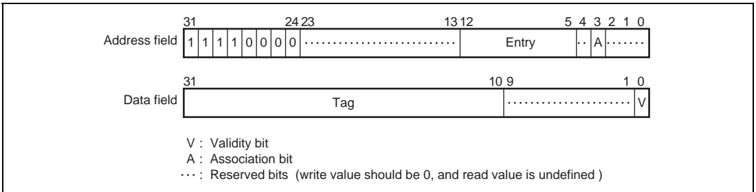
Figure 7.5 Memory-Mapped IC Address Array
