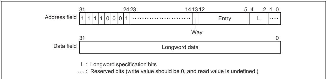
Figure 7.10 Memory-Mapped IC Data Array
