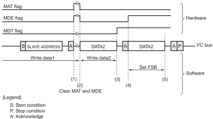
Figure 19.12 Operational Example of Two-byte Data Transmission
