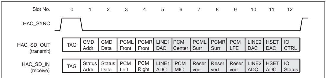
Figure 25.2 AC97 Frame Slot Structure
