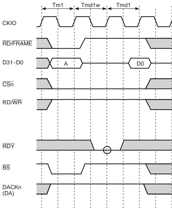
Figure 10.44 MPX Interface Timing 1 (Single Read Cycle, AnW = 0, No External Wait)
