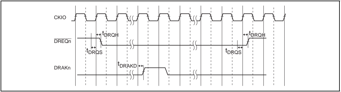
Figure 33.50 \overline{\text{DREQn}}/\text{DRAKn} Timing
