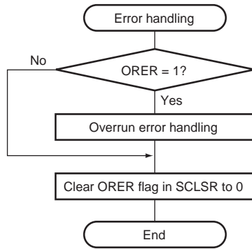
Figure 17.19 Sample Serial Reception Flowchart (2)
