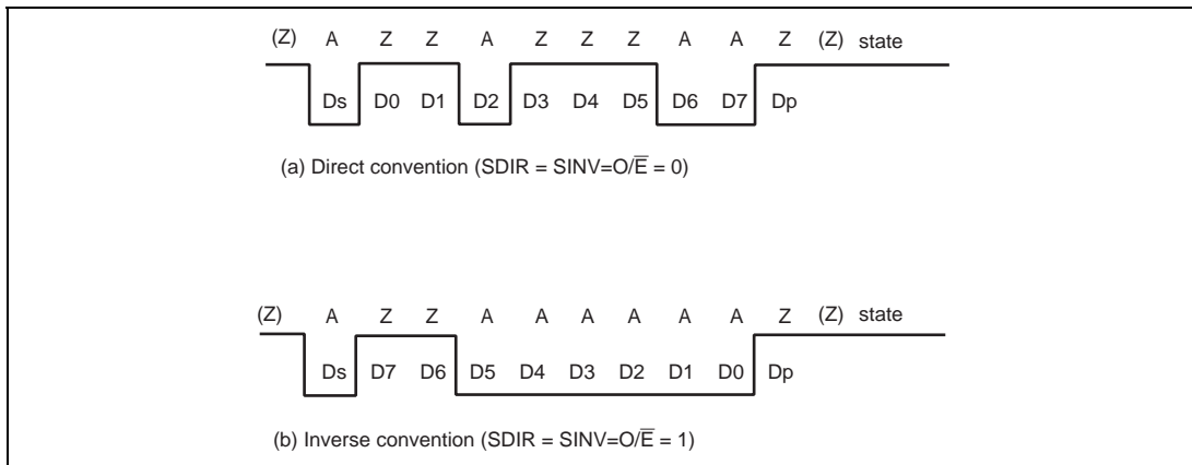
Figure 18.3 Examples of Initial Character Waveforms
