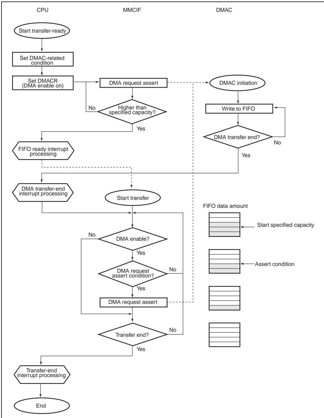
Figure 26.23 Example of Write Sequence Flow
